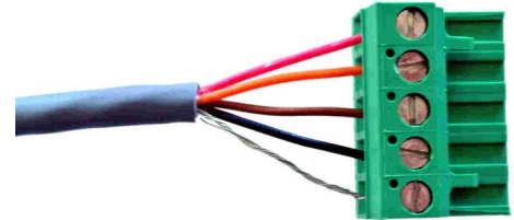
Image 4.2: Wired for Dyacon Control Module
